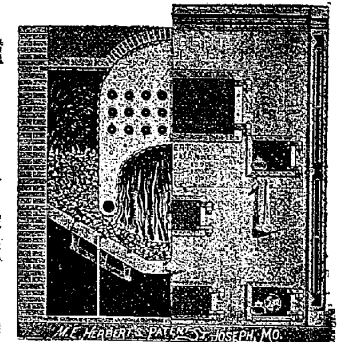
SMOKELESS FURNACE.
