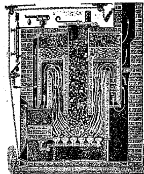
MAGAZINE BOILER.
