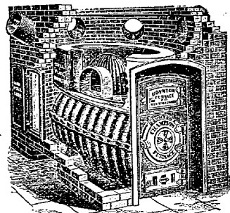
(BRICK-SET OR PORTABLE FORM.)
